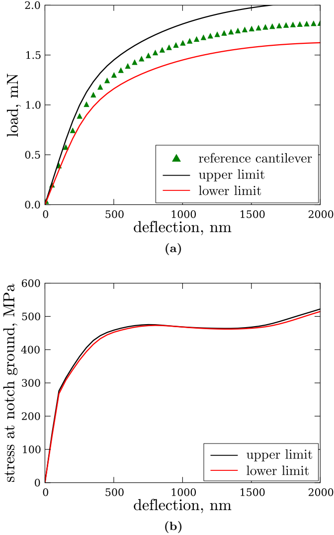
Figure 6.5 (a) Load-deflection response of a cantilever with the dimensions height : width : length = 8.0\ \mu\text{m} : 5.0\ \mu\text{m} : 20.0\ \mu\text{m} together with the upper and lower limits due to deviations in the geometry. (b) Stress at the center of the notch ground for the upper and lower limits.
