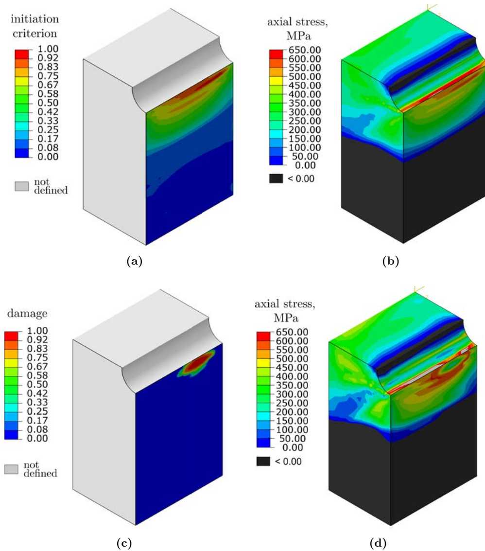
Figure 6.15 Cantilever B: (a) Initiation criterion and (b) stress distribution at the grain boundary at the moment of initiation. (c) Damage and (d) normal stress distribution at the grain boundary for the last increment of the simulation.
